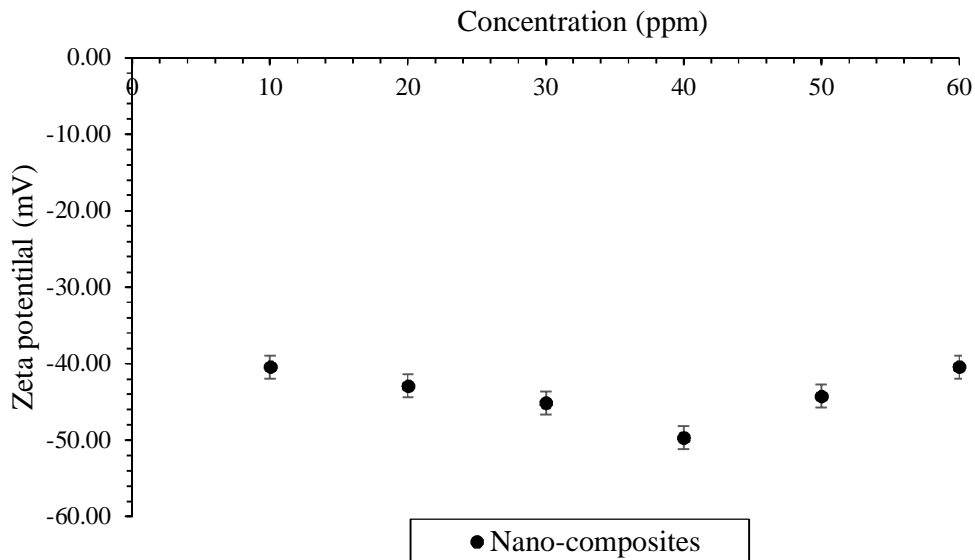
Figure 1. Zeta potential in the presence of nanocomposites
